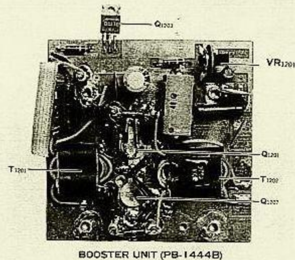
BOOSTER UNIT (PB-1444B)
