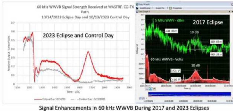
Figure 3 — These plots indicate receiver output, with voltage following signal strength. On the left, Steve Cerwin, WA5FRF, obtained control data (in gray) 1 day prior to the 2023 eclipse, and then he repeated his measurements (in red) on eclipse day. Note the signal enhancement beginning at 1600 UTC and continuing through 1730 UTC. On the right, plots have a similar shape in data recorded during the August 21, 2017, North American total solar eclipse.
