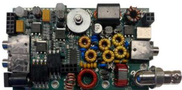
Figure 1 — The QMX main board assembly completed.
