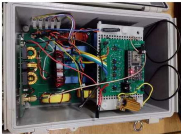
Figure 7 — The complete center unit.
