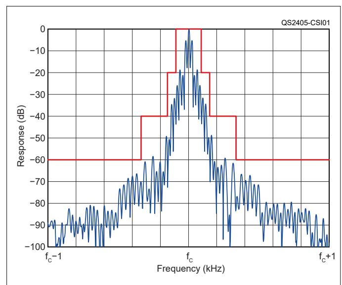
Figure 1 — This graph shows what a clean CW signal would look like (in blue) in relation to the CSI mask (in red). Because no part of the signal exceeds the mask at any point, this transmitter would meet the mask.
