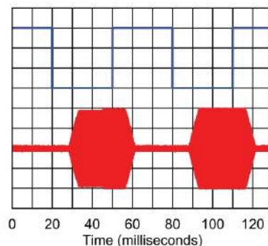
Figure A — CW keying waveform for the Xiegu X6200 showing the first two dits using external keying. Equivalent keying speed is 40 WPM. The upper trace is the key closure; the lower trace is the RF envelope. Horizontal divisions are 20 ms. The transceiver was being operated at 8 W output on the 14 MHz band using QSK set to its default of 100 ms. The first-dit rise time is 4.5 ms; the fall time is 4.3 ms. The second-dit rise time is 4.4 ms; the fall time is 4.3 ms. The first-dit on delay is 10.6 ms; the off delay is 8.9 ms. The second-dit on delay is 10.6 ms; the off delay is 9.0 ms.
