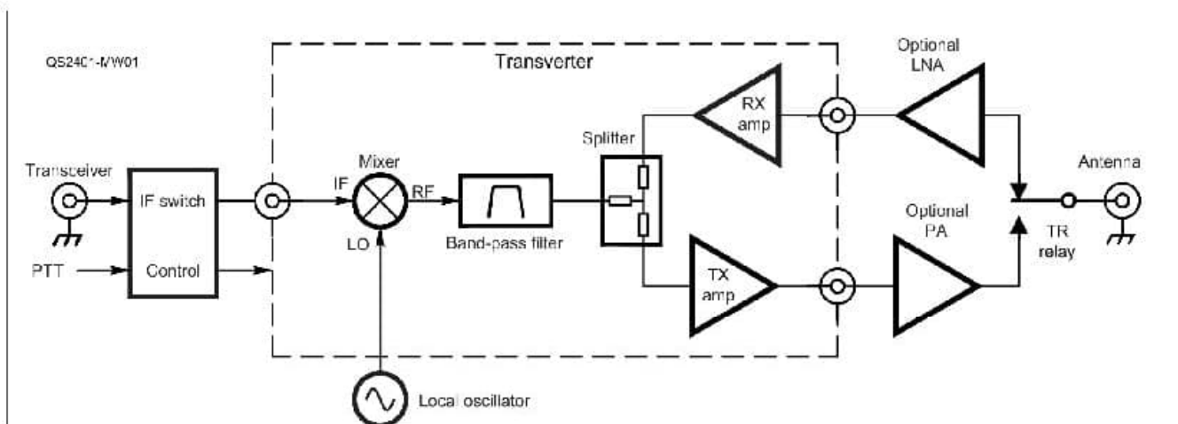
Figure 1 — A block diagram of a simple microwave transverter.
