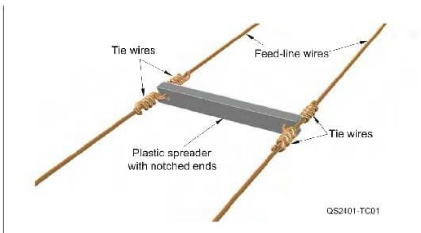
Figure 4 — An alternative approach to using plastic spacers for a 600 \Omega feed line is to notch the ends of the spacers and drill holes near the notches. The feed-line wire is supported by the notches, while short wire ties are threaded through the holes and around the feed line to hold it in place.
