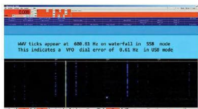
Figure 2 — Checking the variable frequency oscillator (VFO) dial while the radio is in upper sideband (USB) mode.
