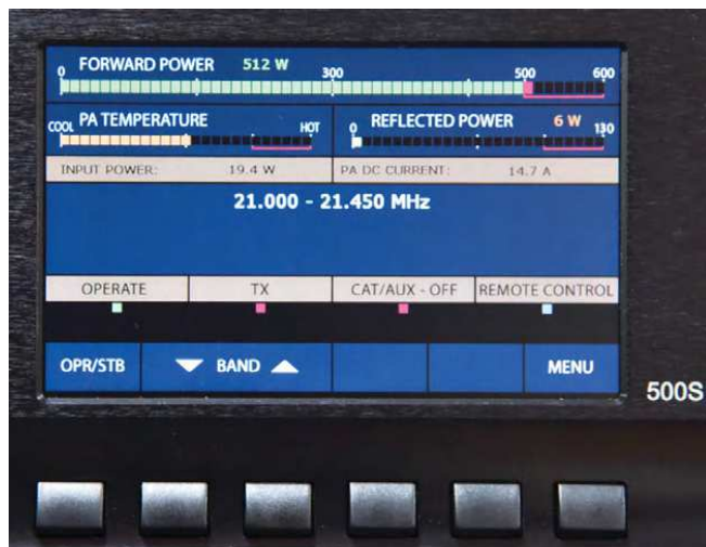
Figure 1 — The main operating screen shows important operating parameters such as selected band, forward and reflected power, drive power, and PA temperature. It's not a touchscreen — selections are made using the buttons below the screen. The MENU button at the lower right brings up various setup and monitoring screens.
