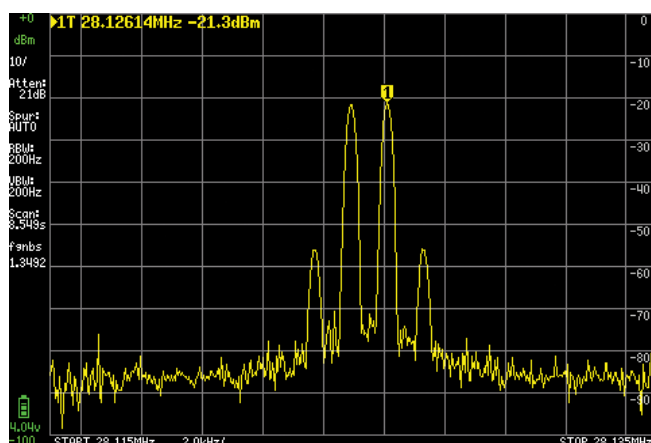
Figure 9 — The 10-meter two-tone transverter's input.
