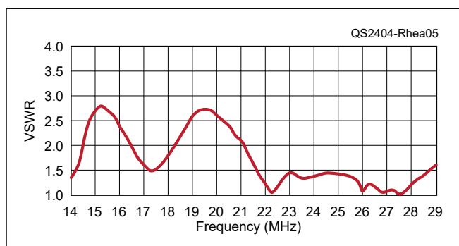
Figure 4 — VSWR of the LPDA through TMR-400 coax at the tower base.
