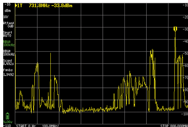
Figure 11 — The tinySA Ultra 0 – 800 MHz spectrum at the TV antenna feed.
