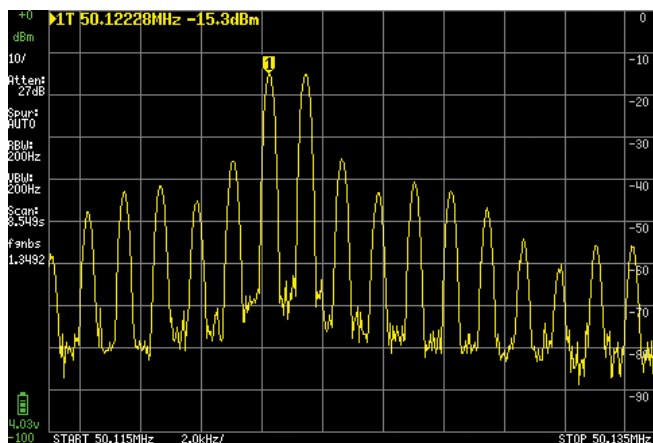
Figure 10 — The resultant 6-meter two-tone spectrum.
