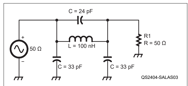
Figure 4 — A schematic of the Cauer low-pass filter.
