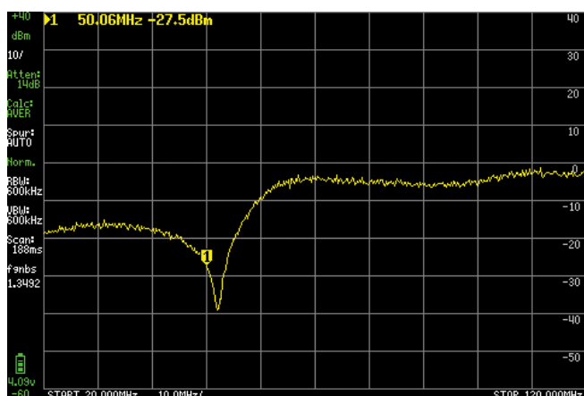
Figure 8 — The terminated filter's return loss.
