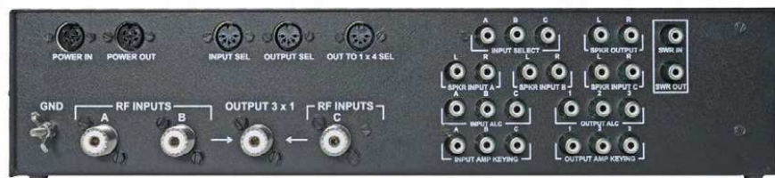
Figure 5 — The W2IHY 3 × 4 Switch Plus controller rear panel.
