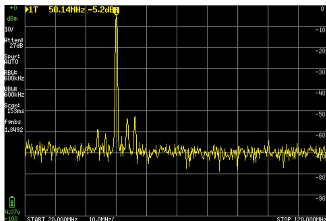
Figure 7 — The filtered transverter's output.
